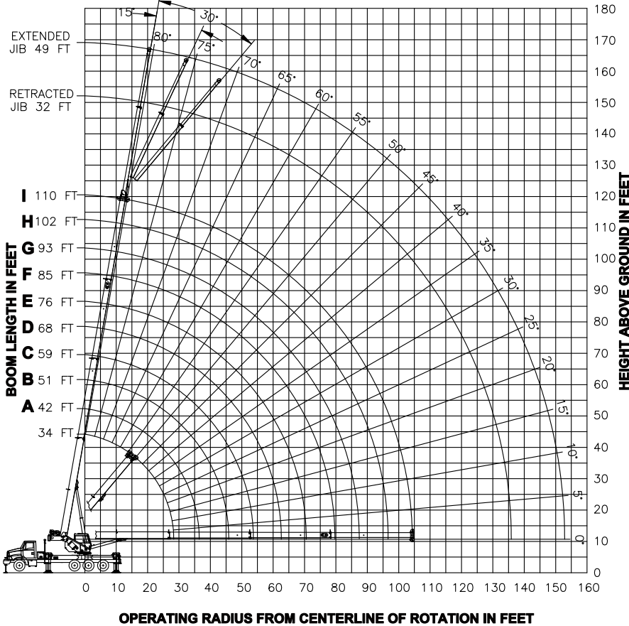
- RANGE DIAGRAM -
