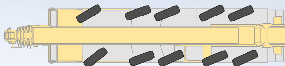
Variable steering concept Concept de direction variable
